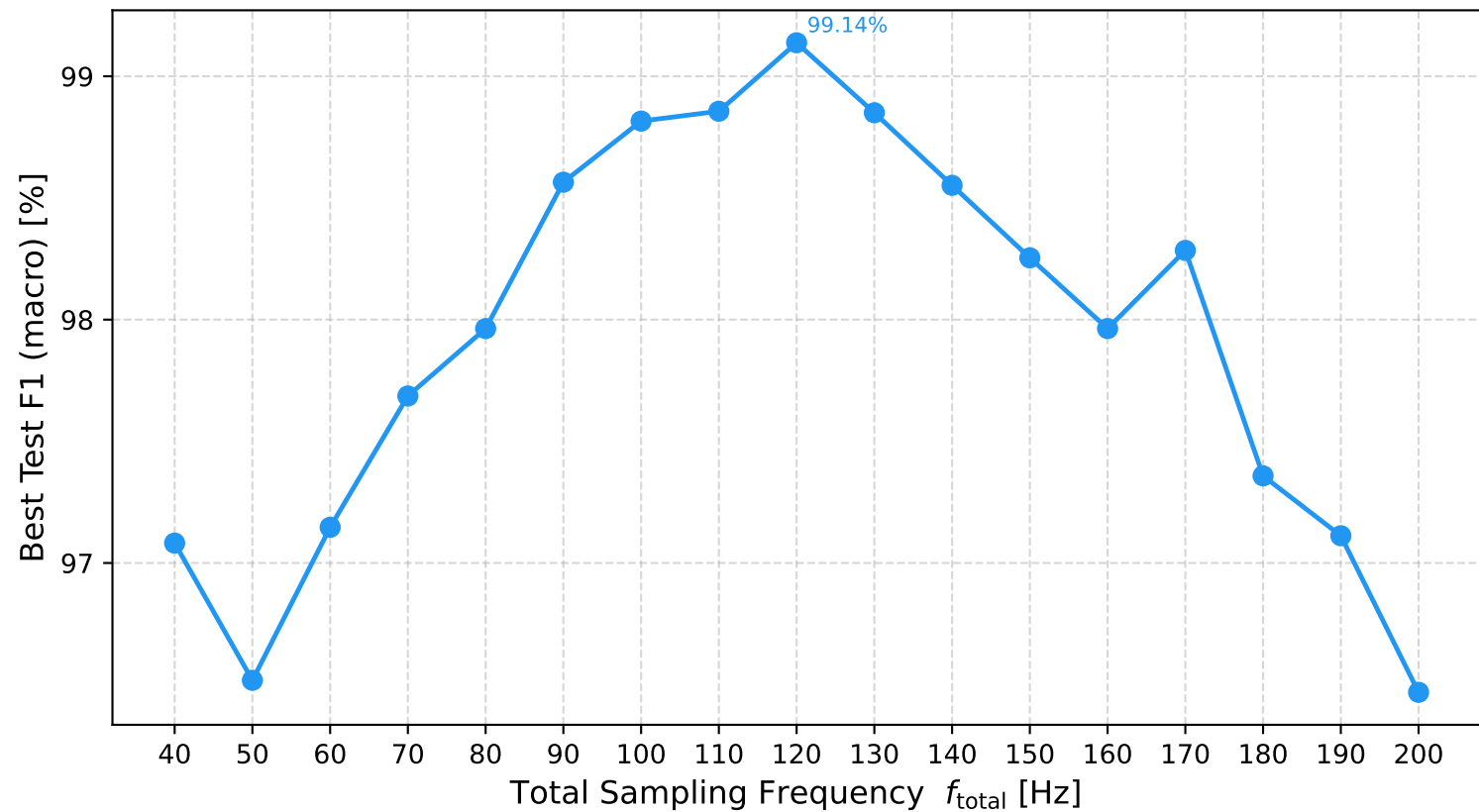
Pareto Curve: Best F1 vs. Total Sampling Frequency (Clean→Clean)
